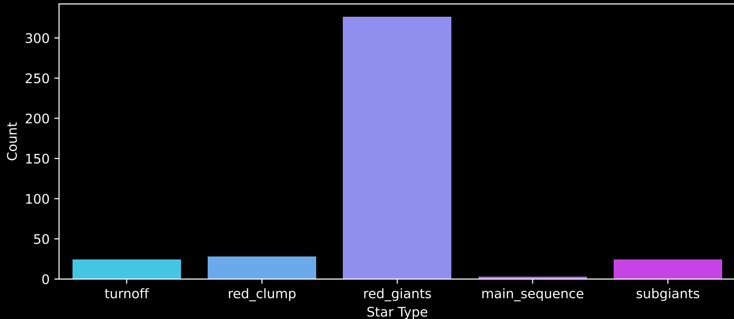
APOGEE DR17 Field: [000-04] Count plot of Star Type
