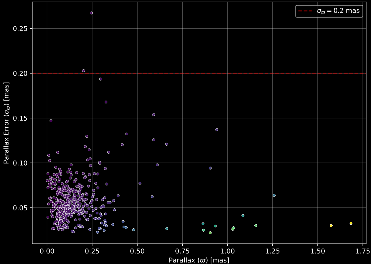
APOGEE DR17 Field: [000-04] Parallax Quality (n= 405)
