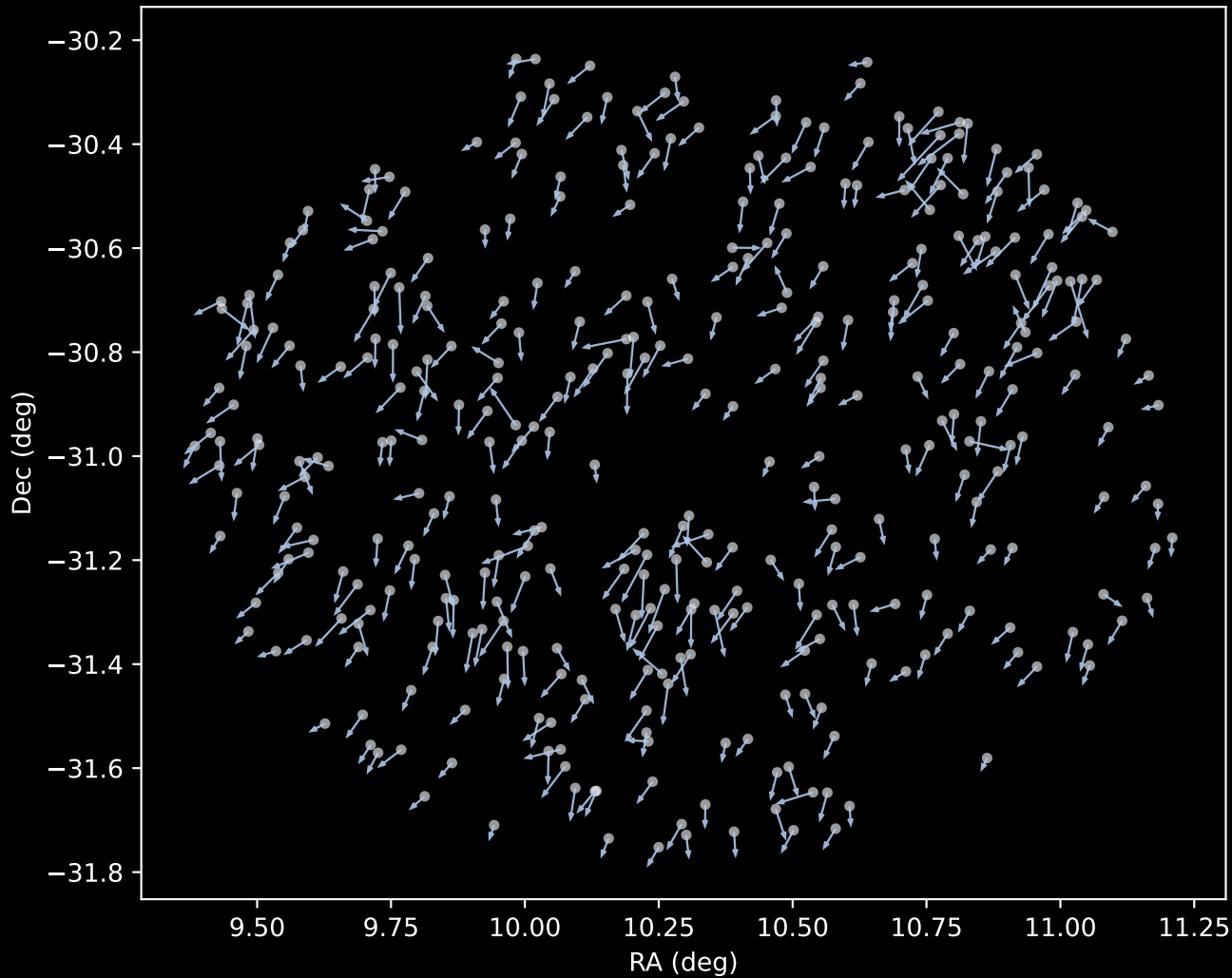
APOGEE DR17 Cluster 1 Proper Motion Vectors (n=365)
