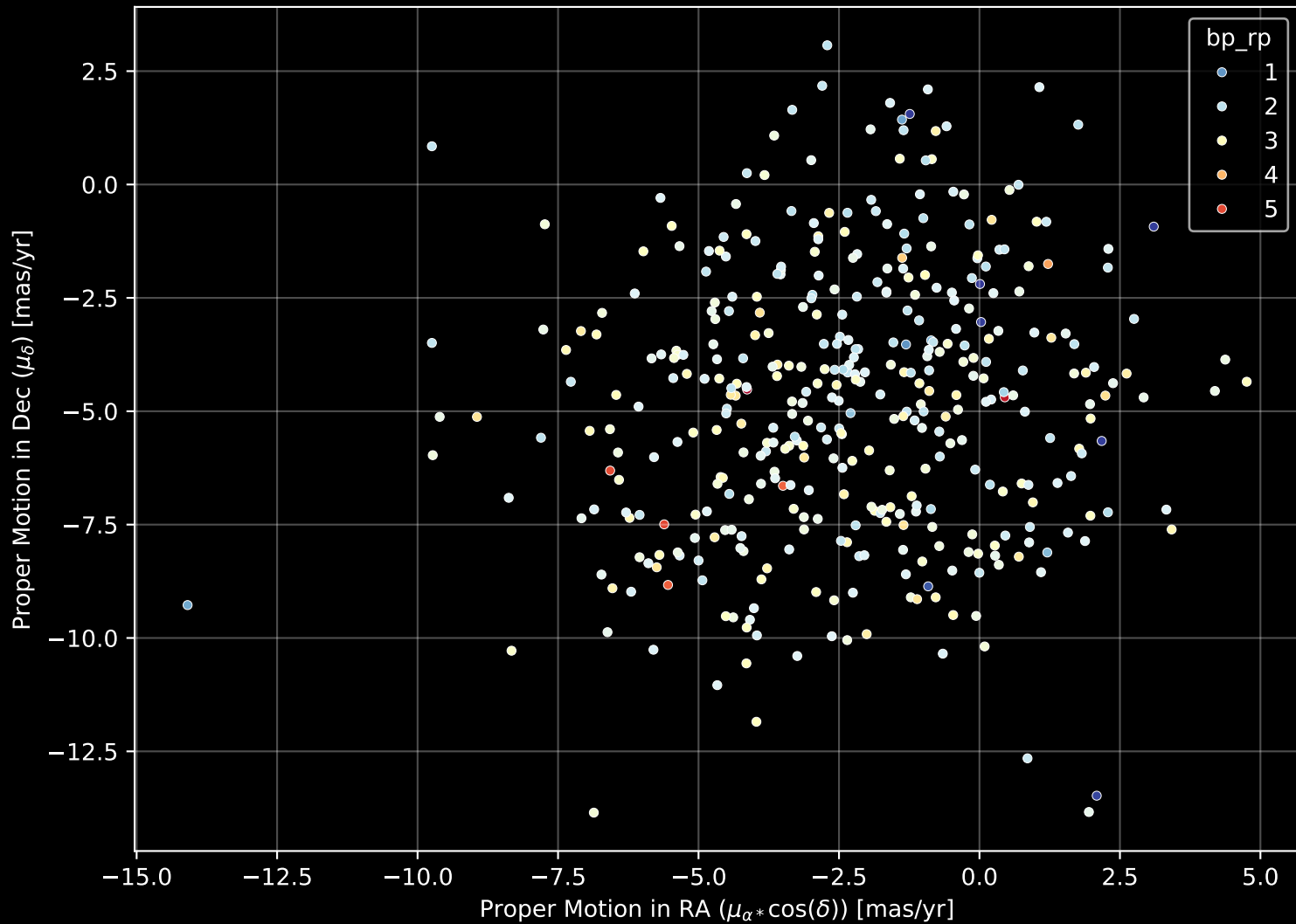
APOGEE DR17 Field: [000-04] Proper Motion Diagram (n= 405)
