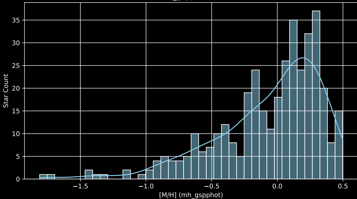
APOGEE DR17 Field: [000-04 [M/H] (mh_gspphot) (n= 375)
