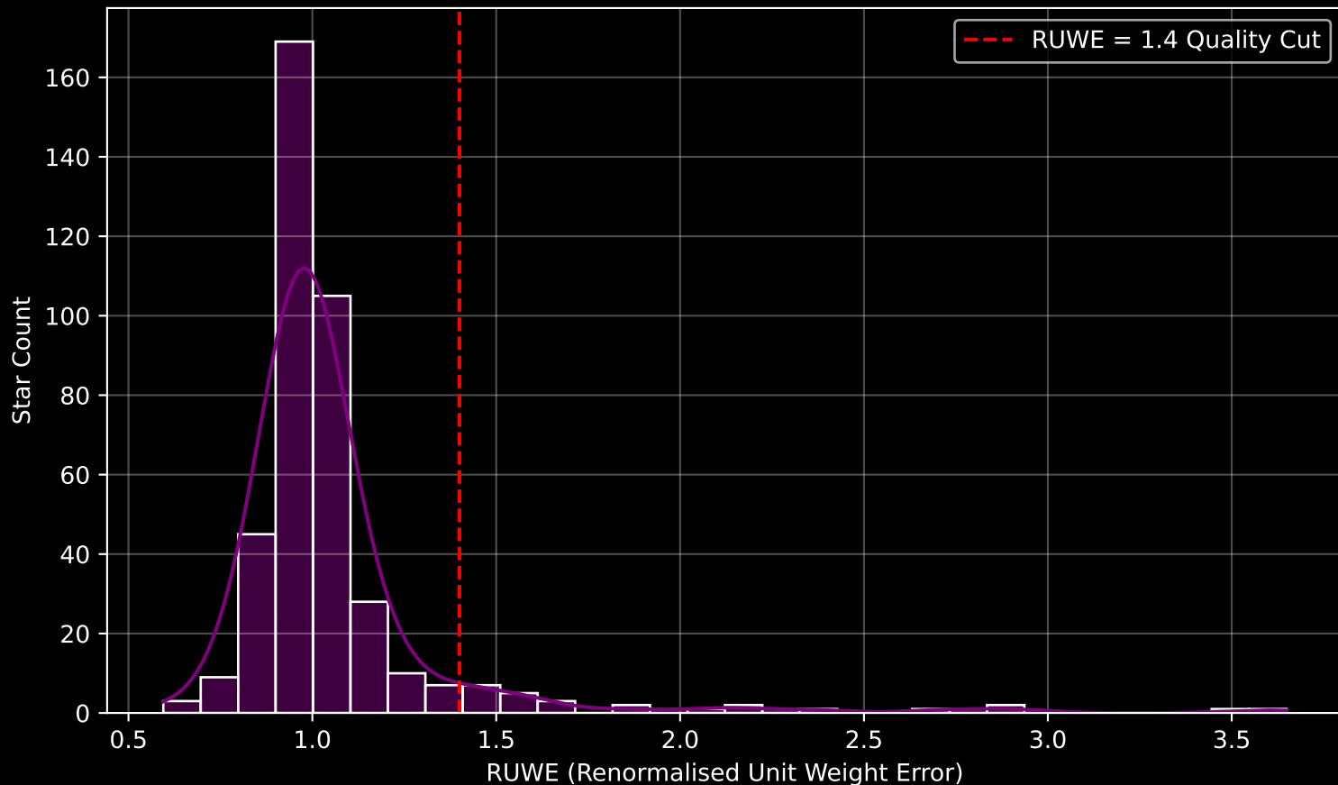
GAPOGEE DR17 Field [000-04] RUWE Distribution (n= 404)
